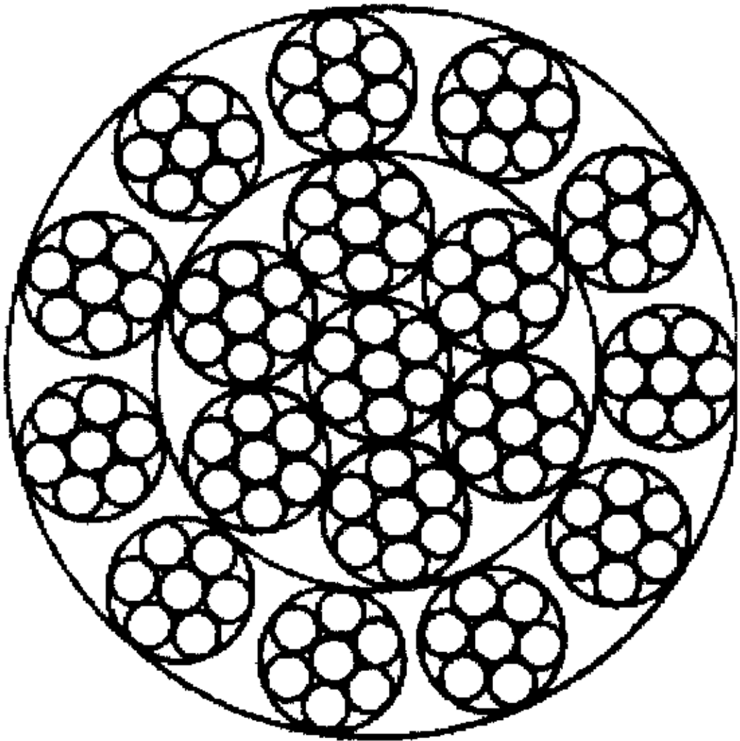
17×7+IWS
