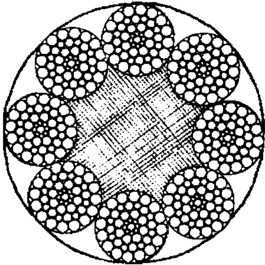
8×49SWS+FC
