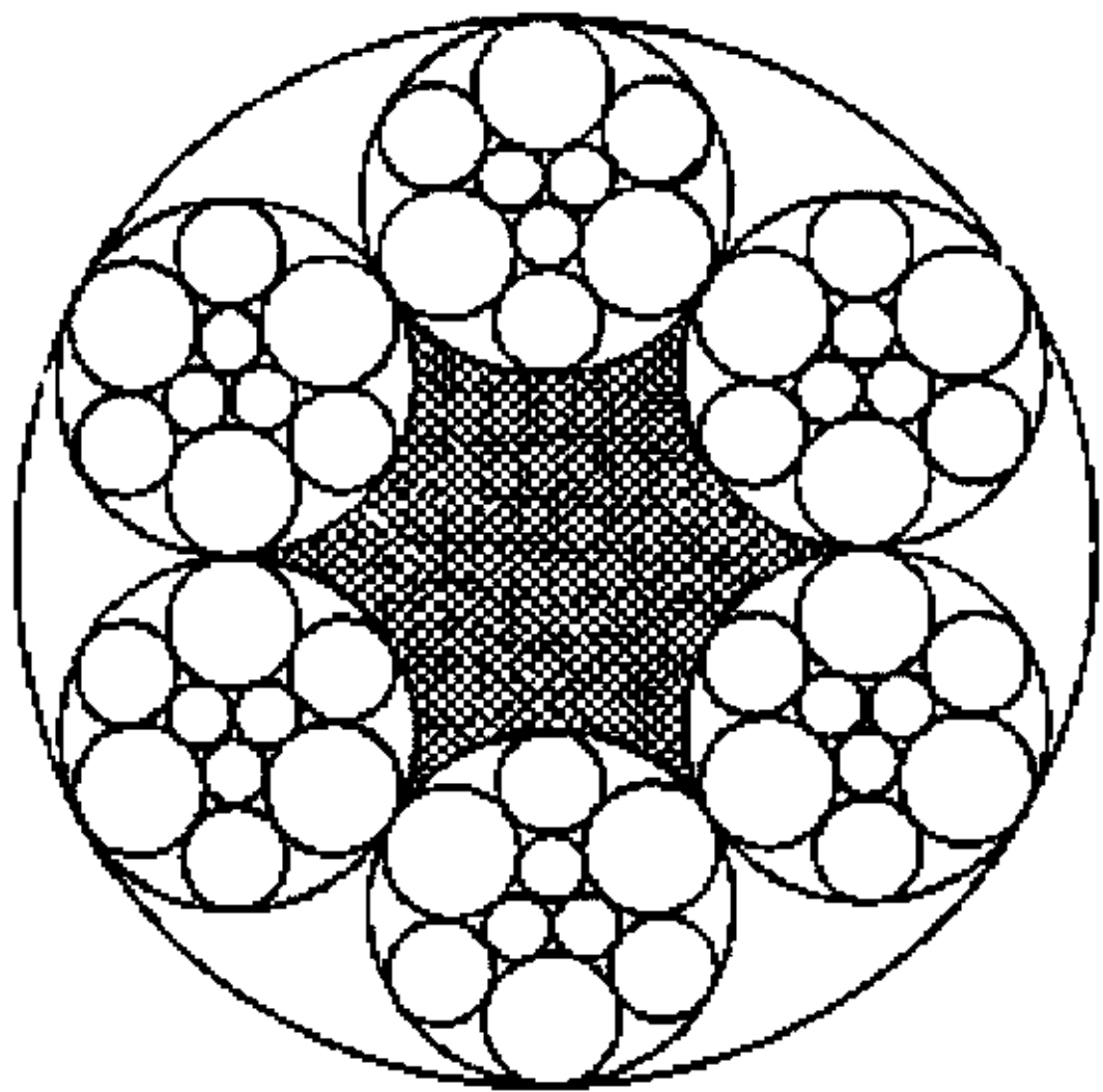
6×9W-FC
