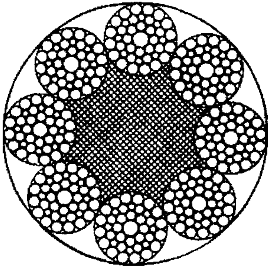
8×41WS+FC
