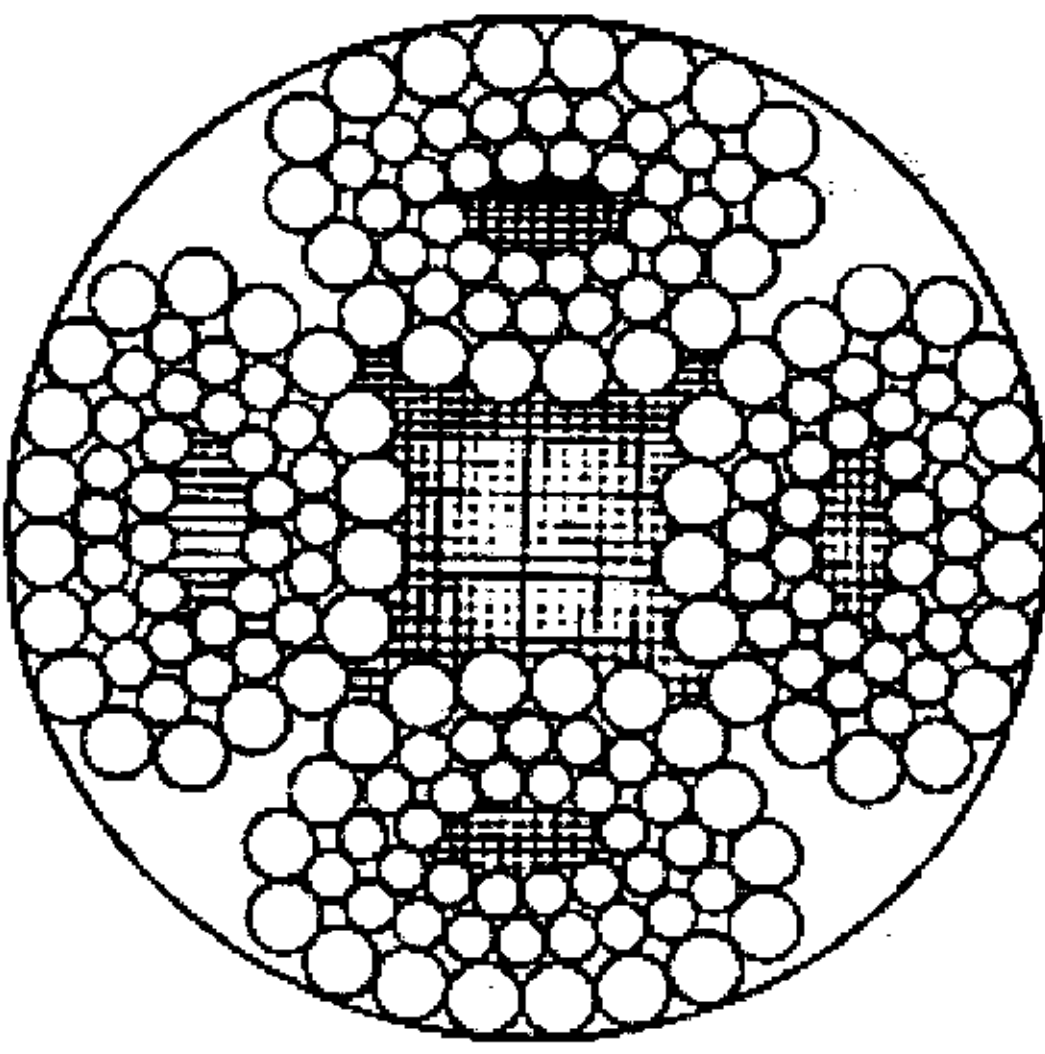
4V×48S+5FC
