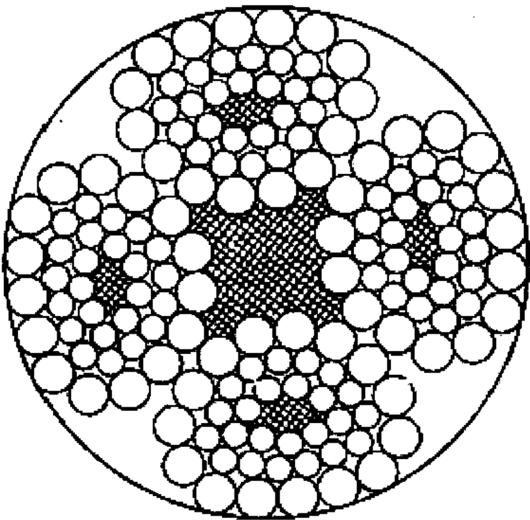
4V×39S+5FC
