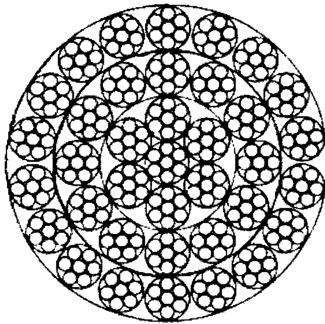
36×7+IWS
