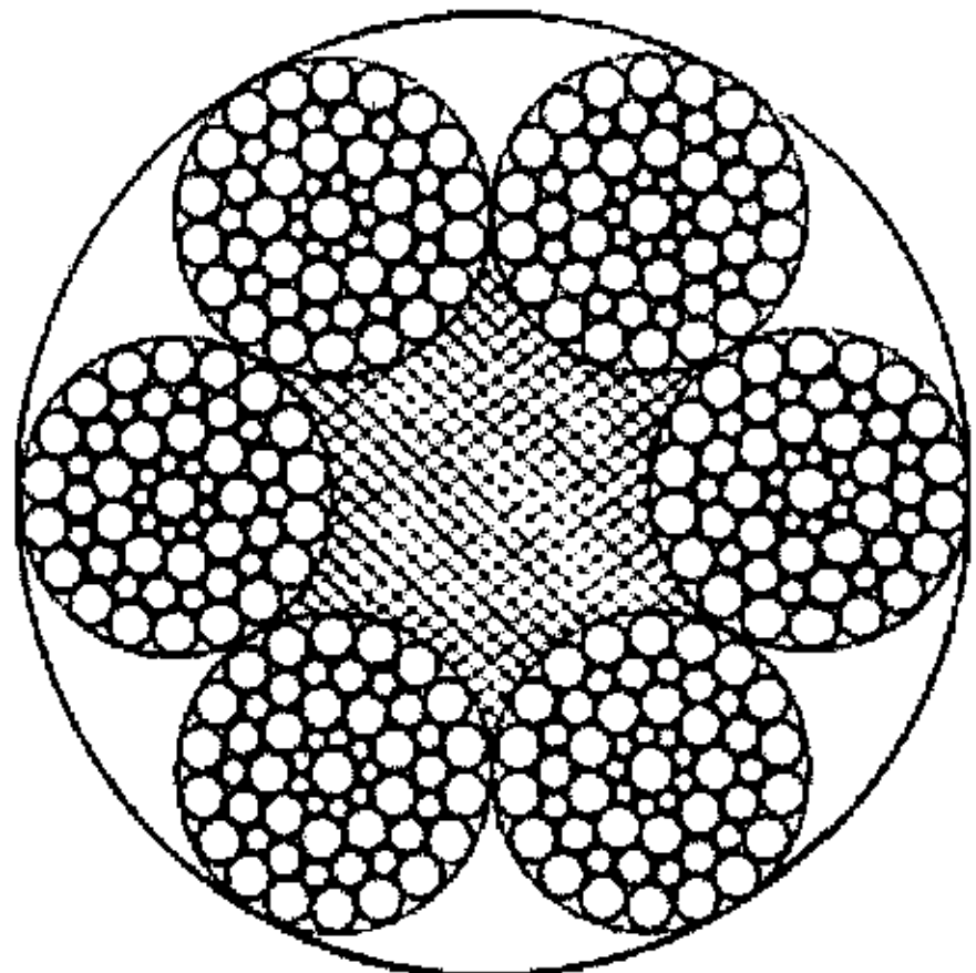
6×55SWS+FC
