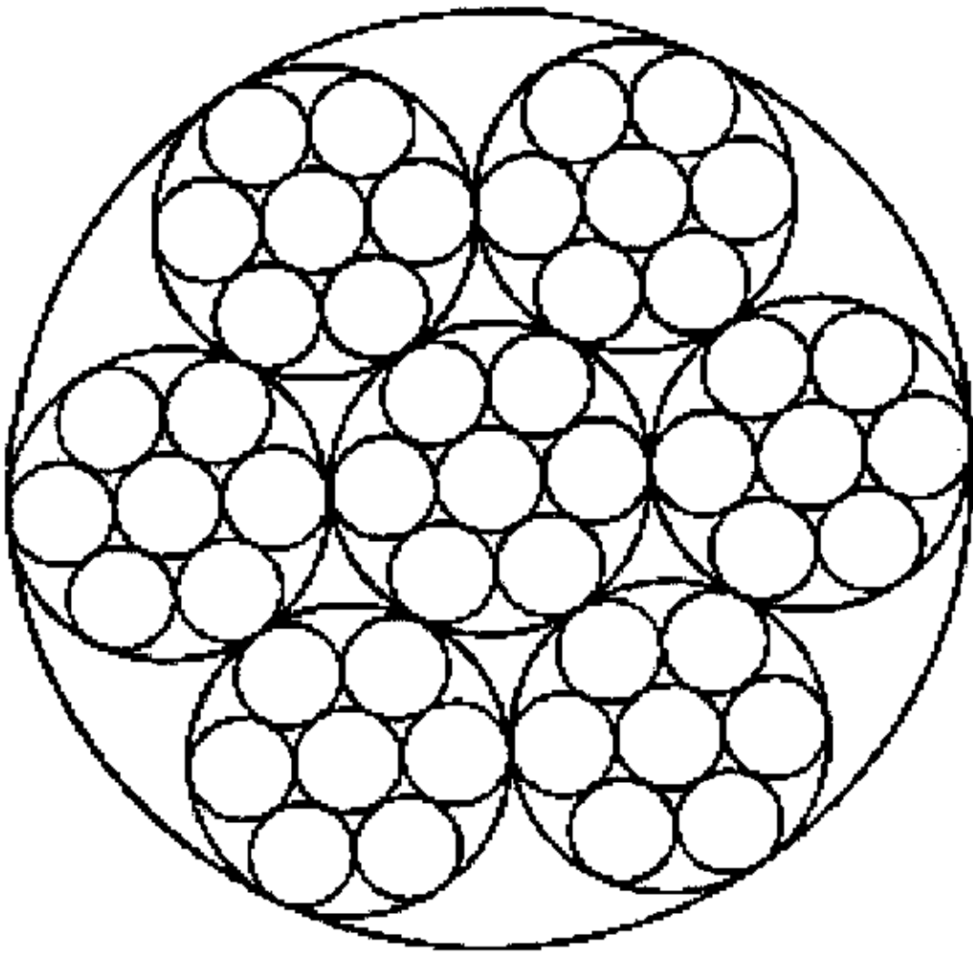
6×7+IWS
