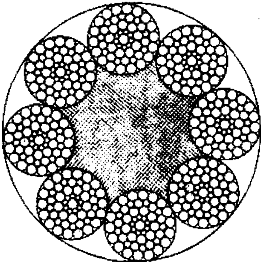
8×55SWS+FC
