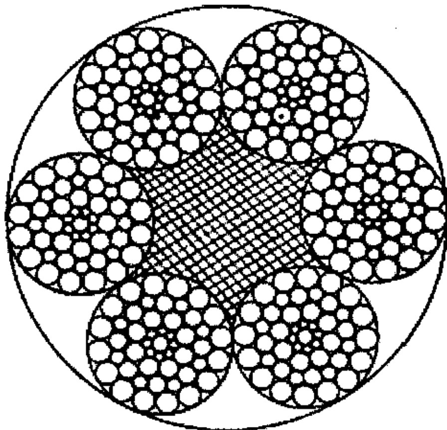
6×49SWS+FC
